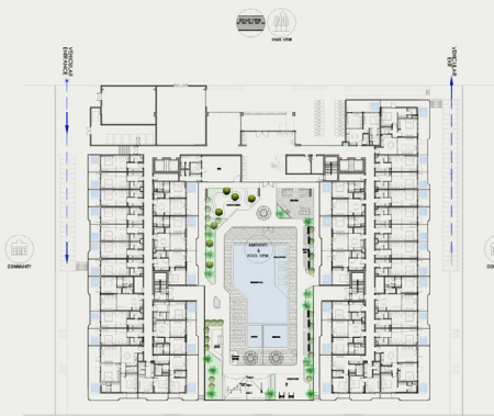
Ground Floor Plan Key Plan
